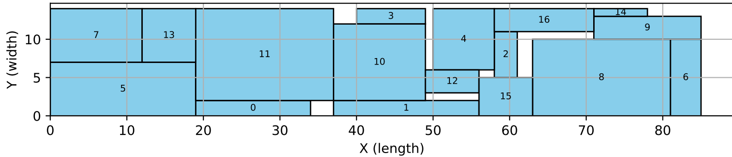
17_7 | reagg_tres | MIP
