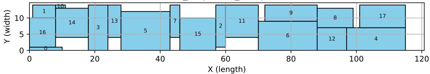
18_10 | reagg_tres | MIP
