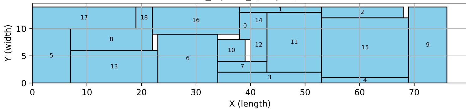
19_8 | tres_sym | bigm
