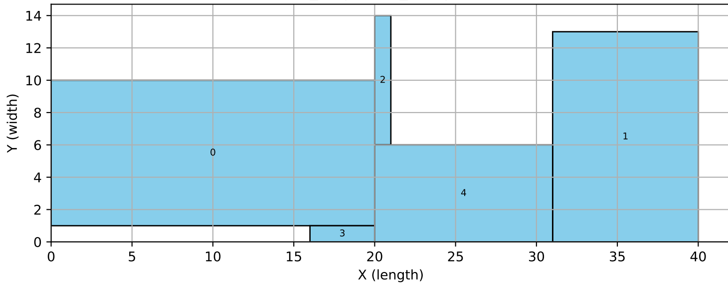
5_10 | reagg_tres | MIP
