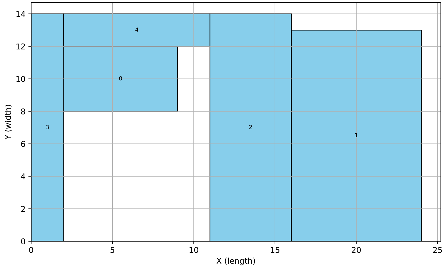
5_6 | traditional | bigm
