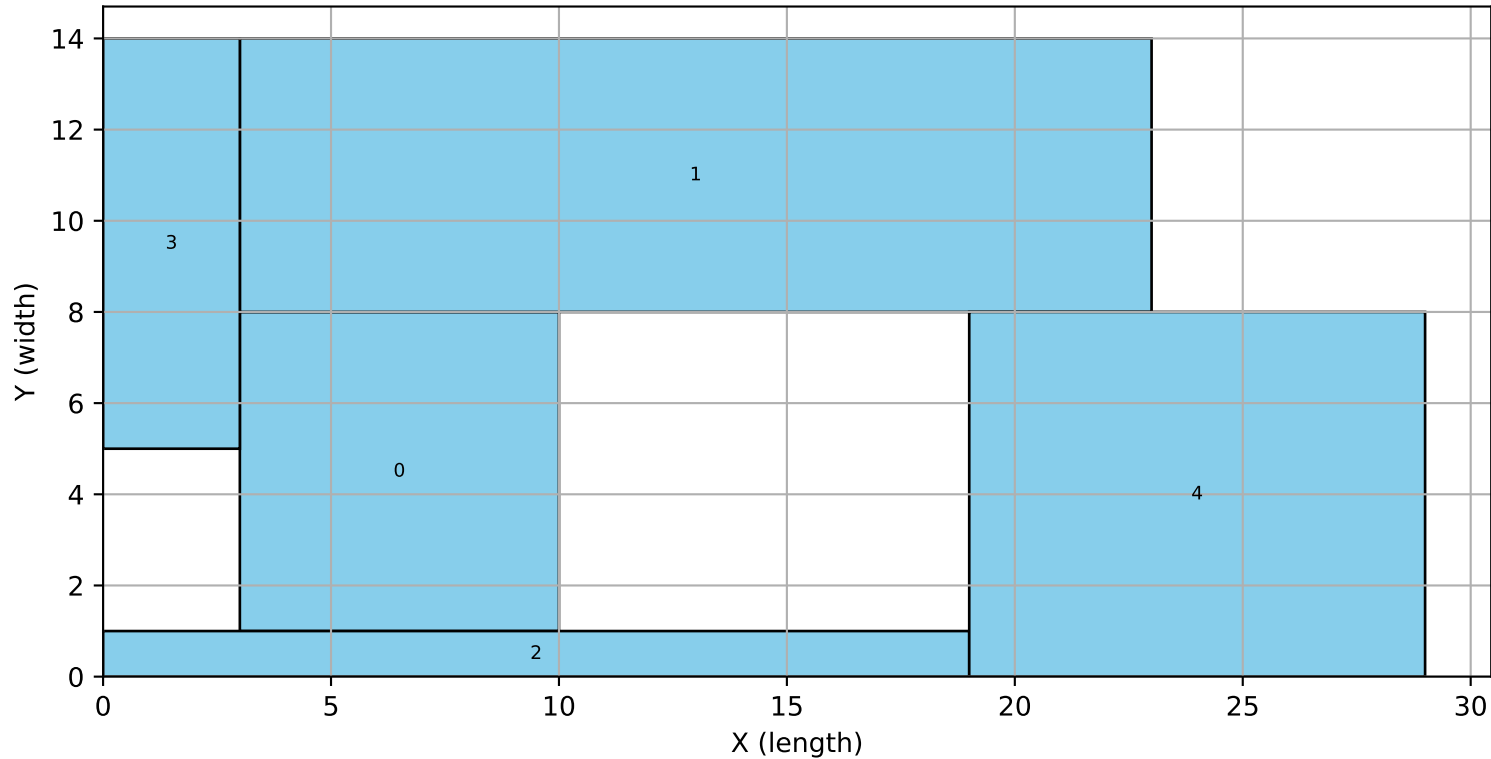
5_8 | traditional | bigm
