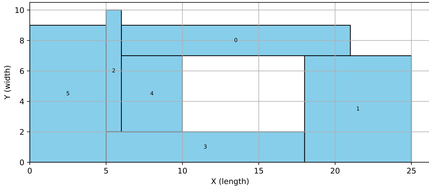
6_1 | traditional | bigm
