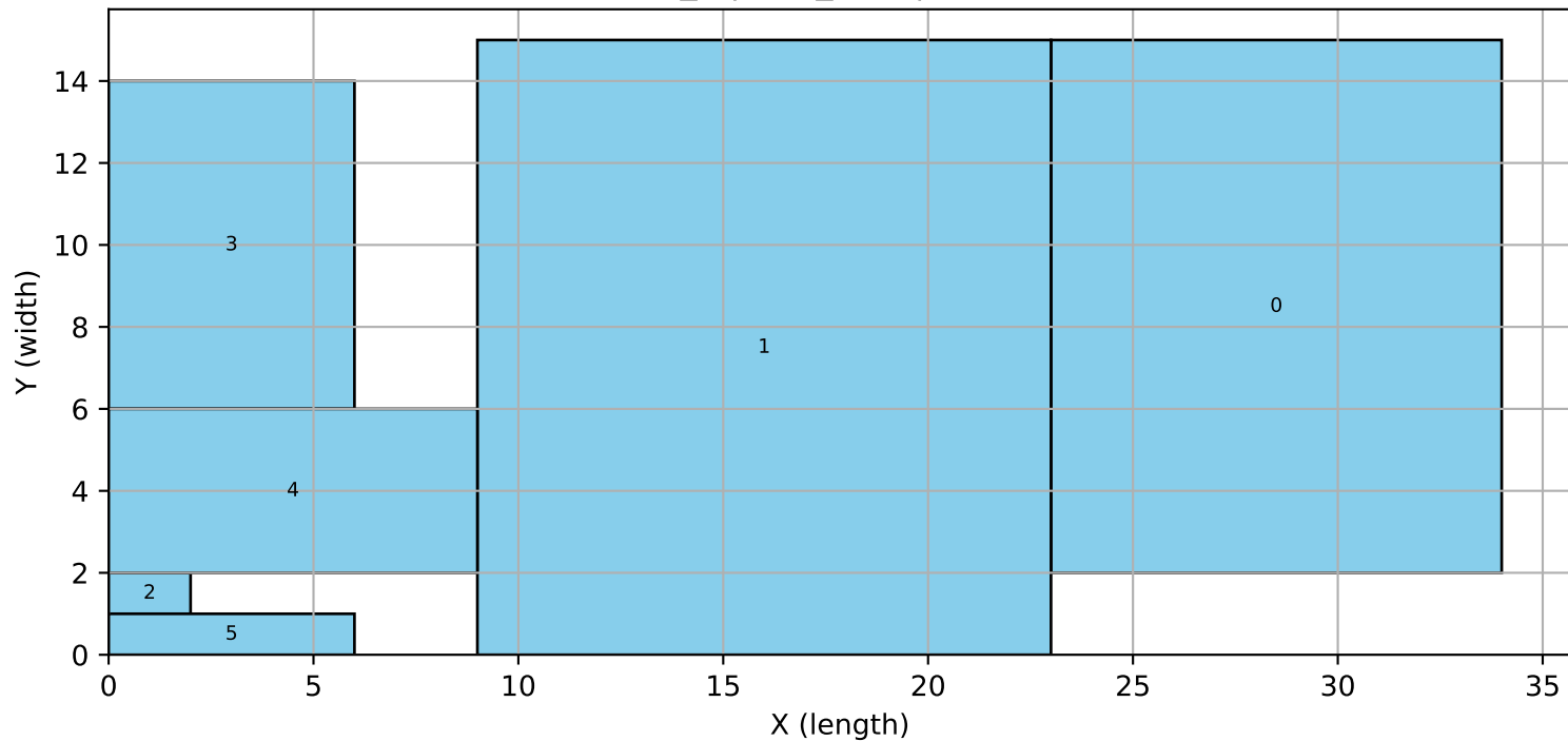
6_3 | tres_sym | bigm
