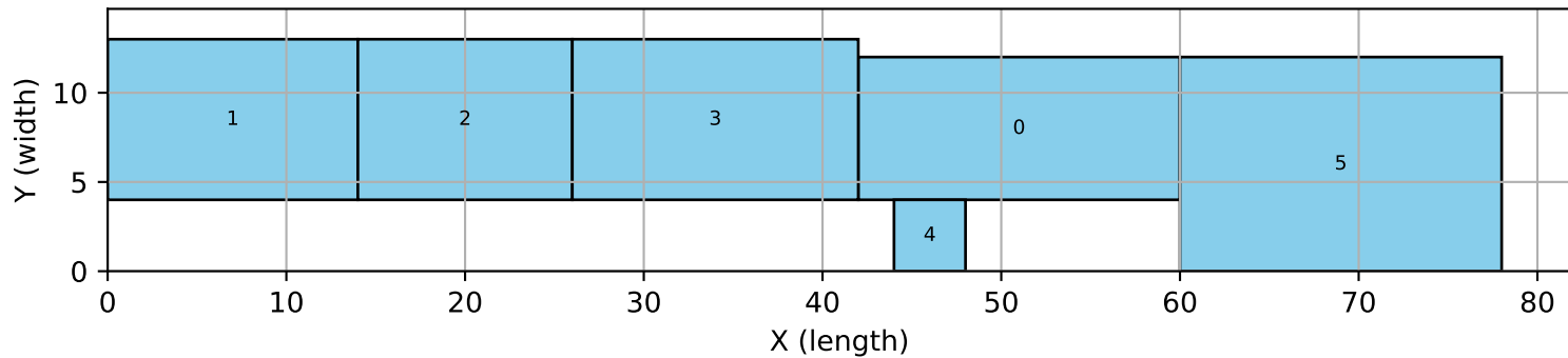
6_6 | tres_sym | bigm
