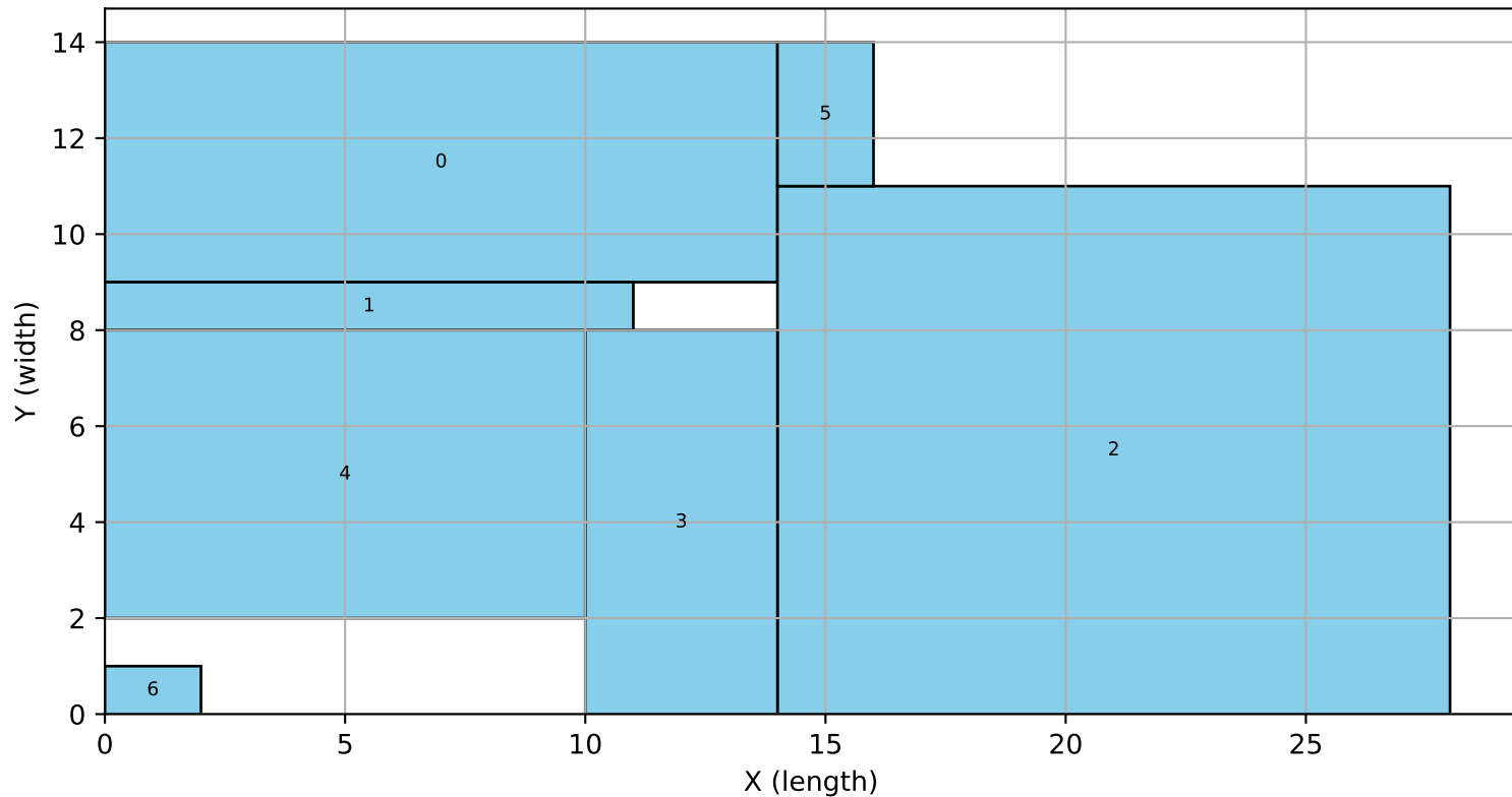
7_7 | traditional | bigm
