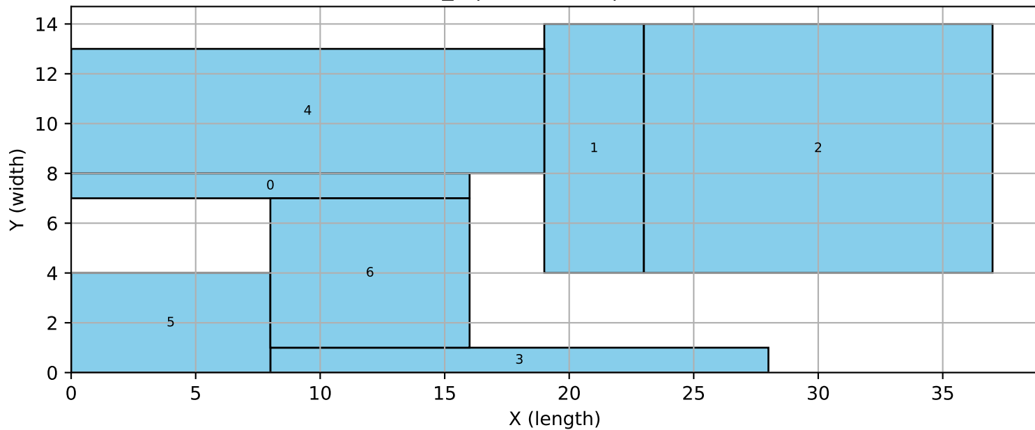
7_8 | traditional | bigm
