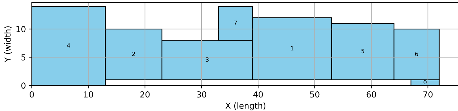
8_10 | reagg | MIP
