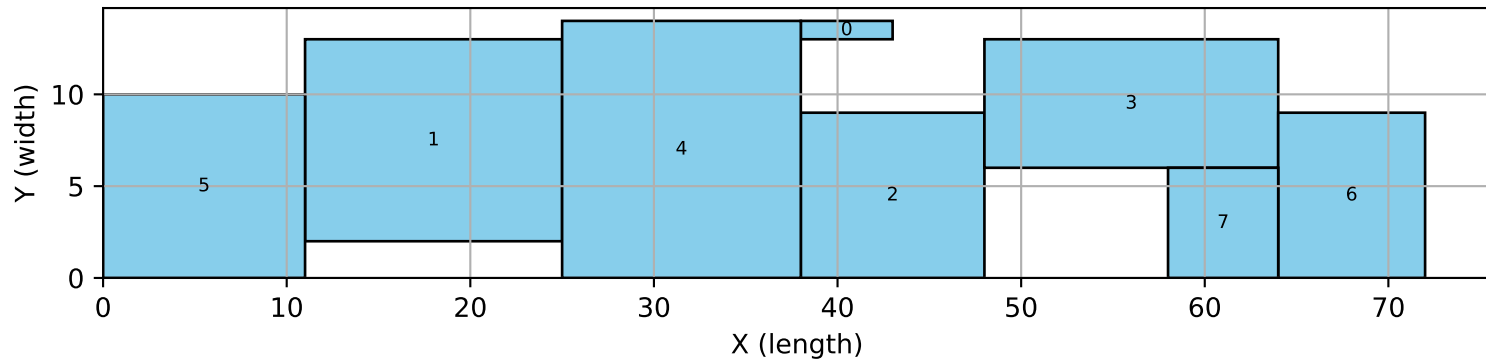
8_10 | tres_sym | bigm
