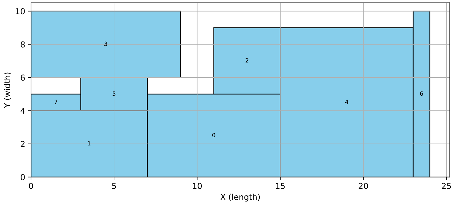
8_1 | tres_sym | hull
