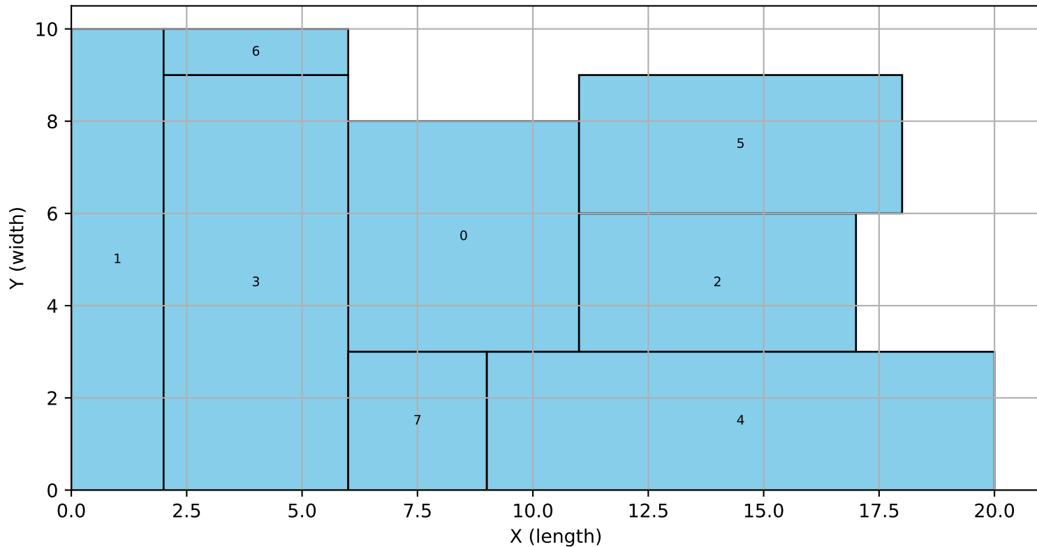
8_2 | altered | bigm
