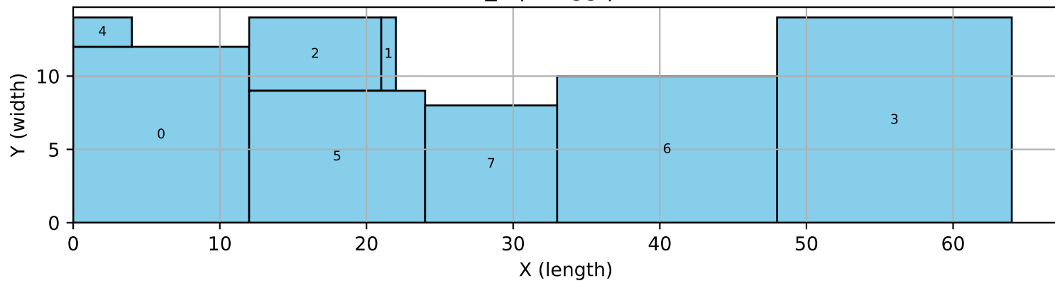
8_4 | reagg | MIP
