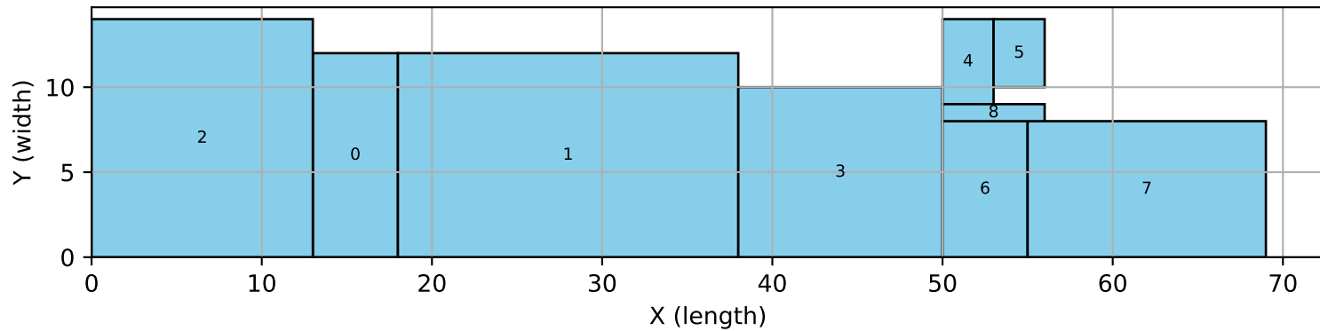
9_6 | tres_sym | hull
