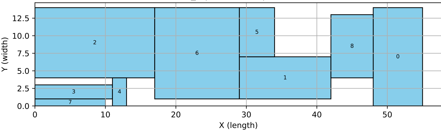
9_9 | traditional | bigm
