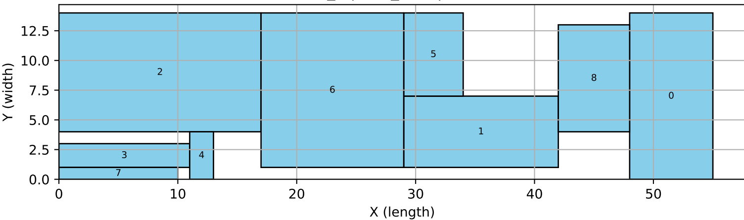
9_9 | tres_sym | bigm
