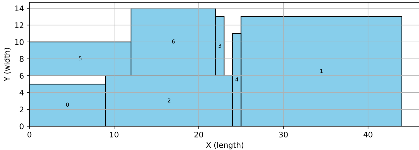
7_10 | tres | bigm
