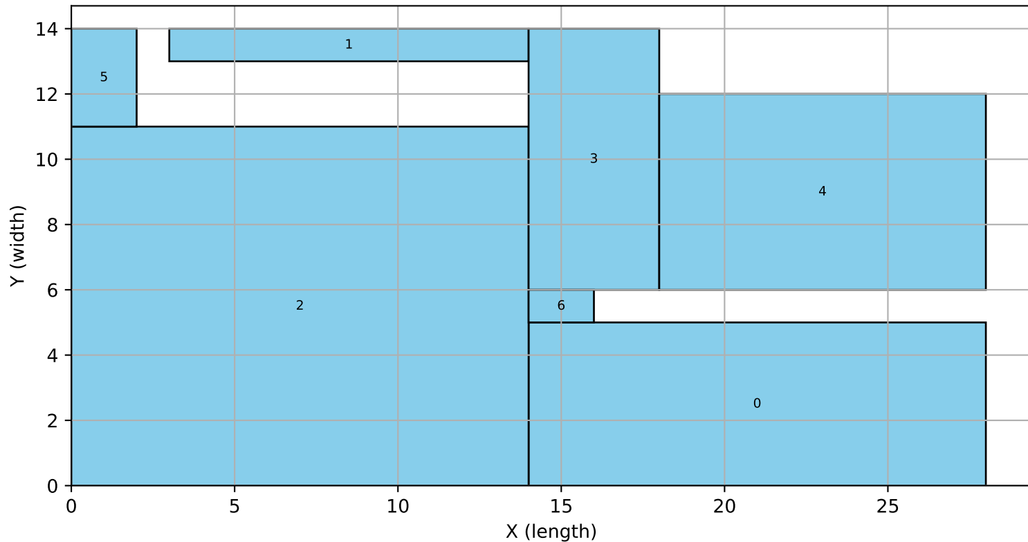
7_7 | reagg_tres | MIP
