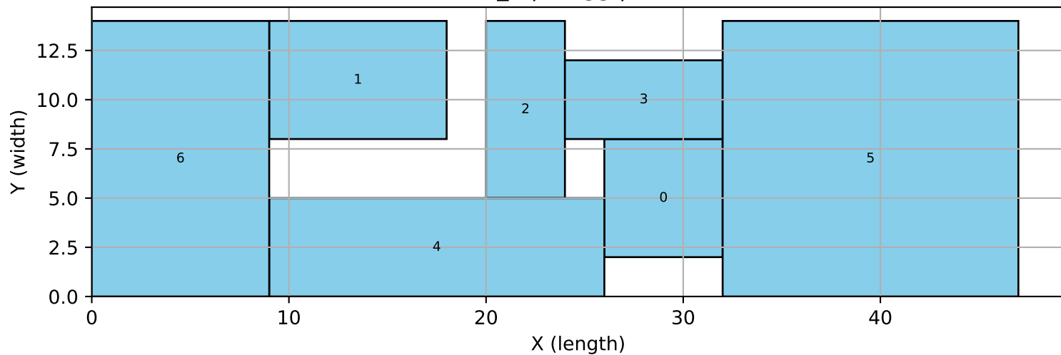
7_9 | reagg | MIP
