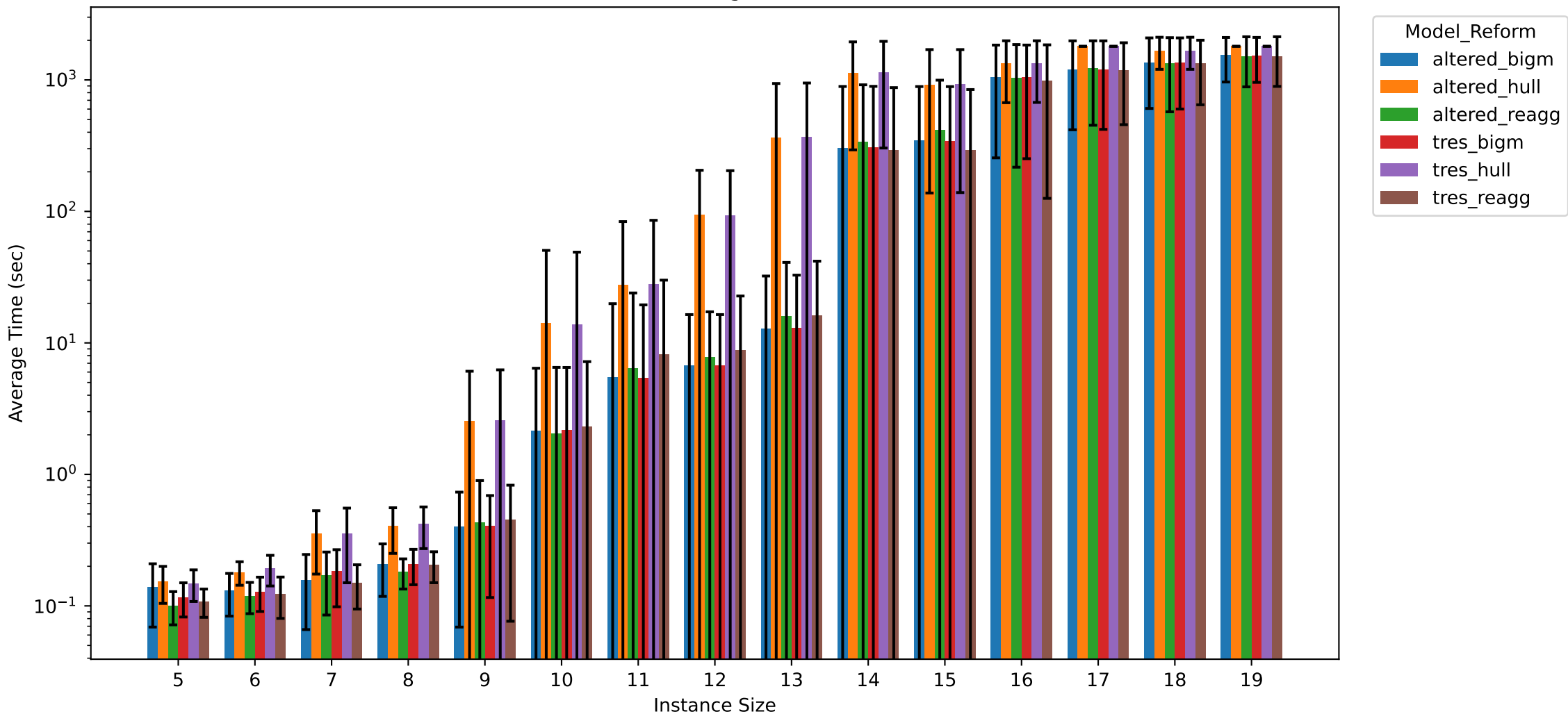
Average Solve Time by Size & Reformulation (5 Cases Averaged, \pm 1 std)
