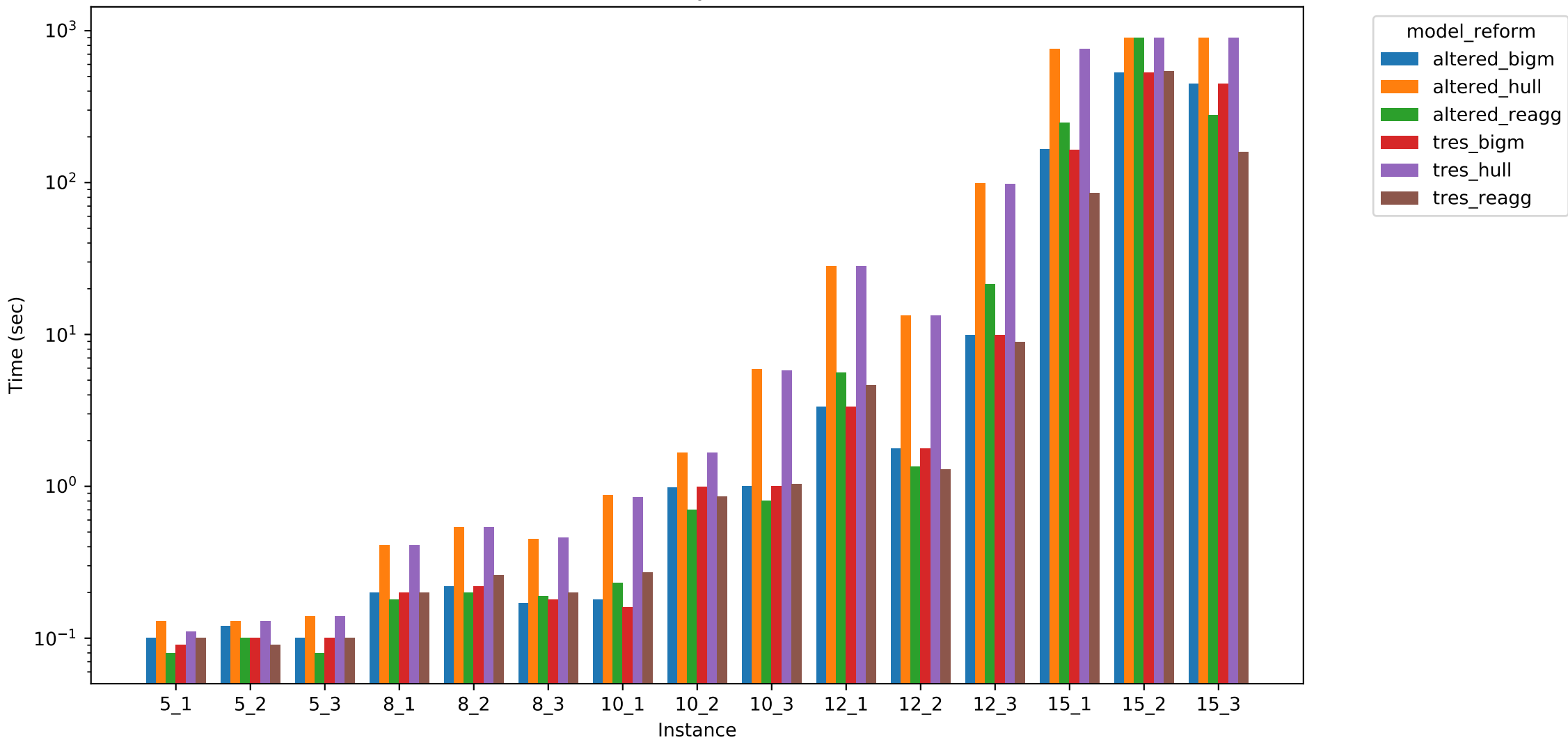
Benchmark Run Times by Model & Reformulation
