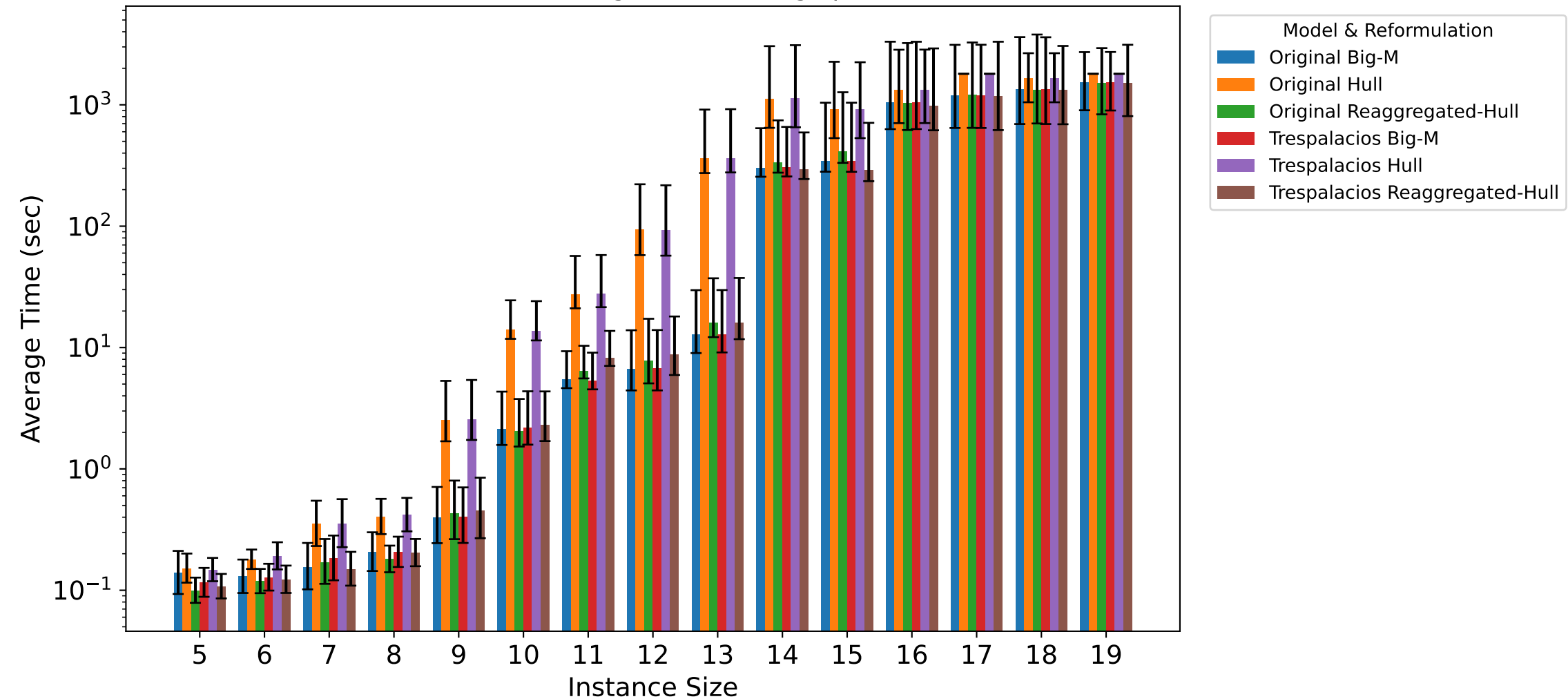
Average Solve Time by Size & Reformulation (10 Cases Averaged, \pm 1\sigma in log-space)
