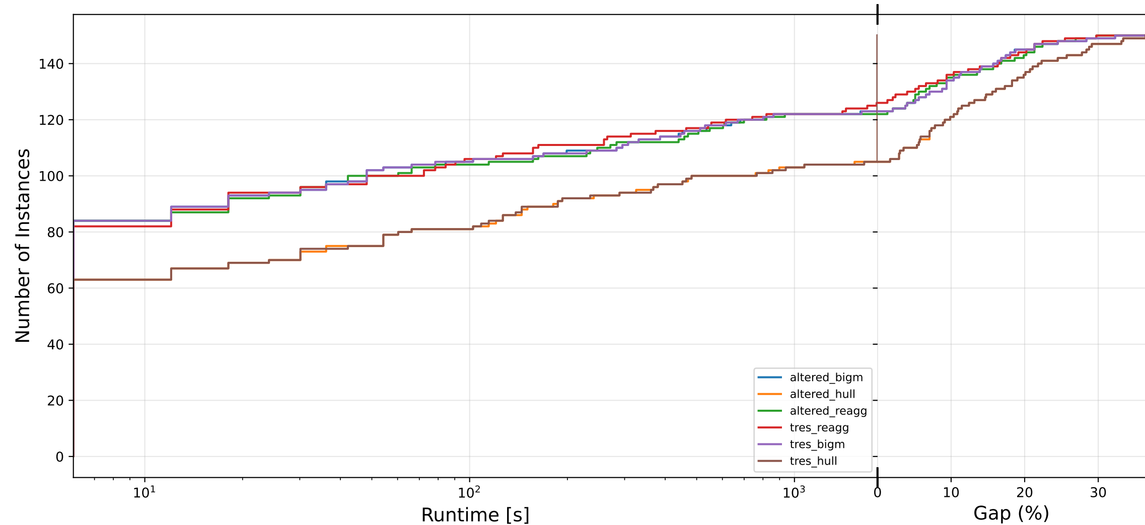
Absolute Performance Profile
