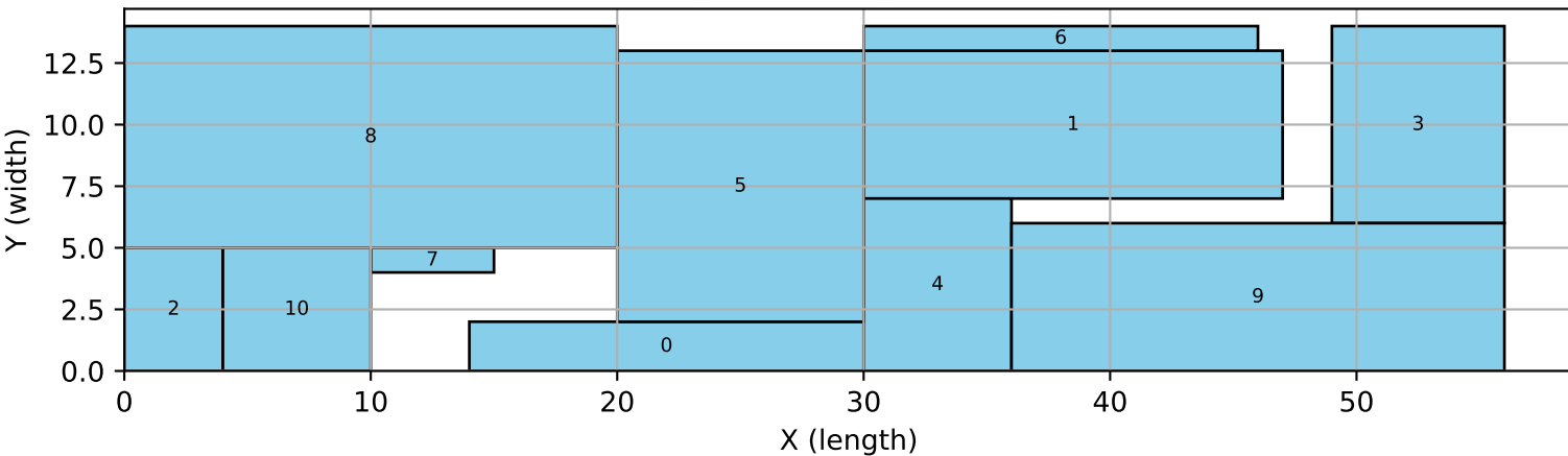
11_10 | reagg_tres | MIP
