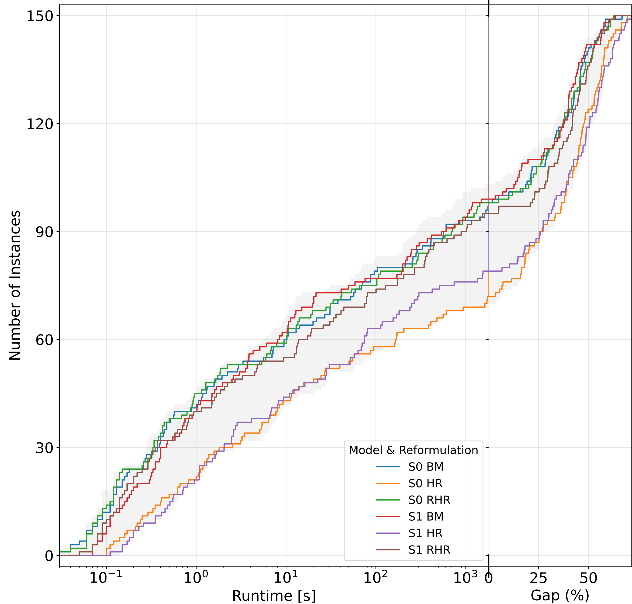
Absolute Performance Profile of Strip Packing Problem using HiGHS
