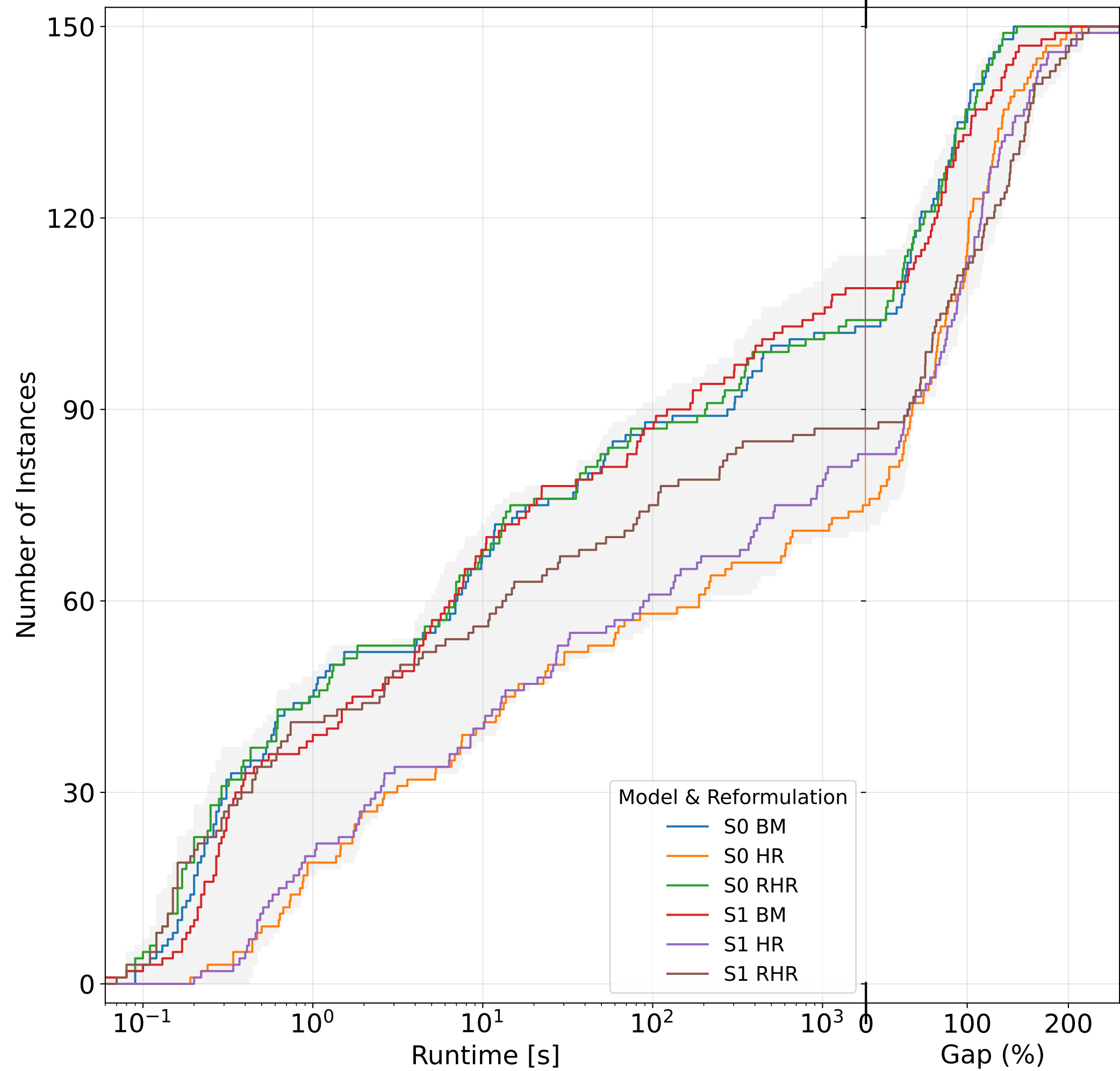
Absolute Performance Profile of Strip Packing Problem using SCIP
