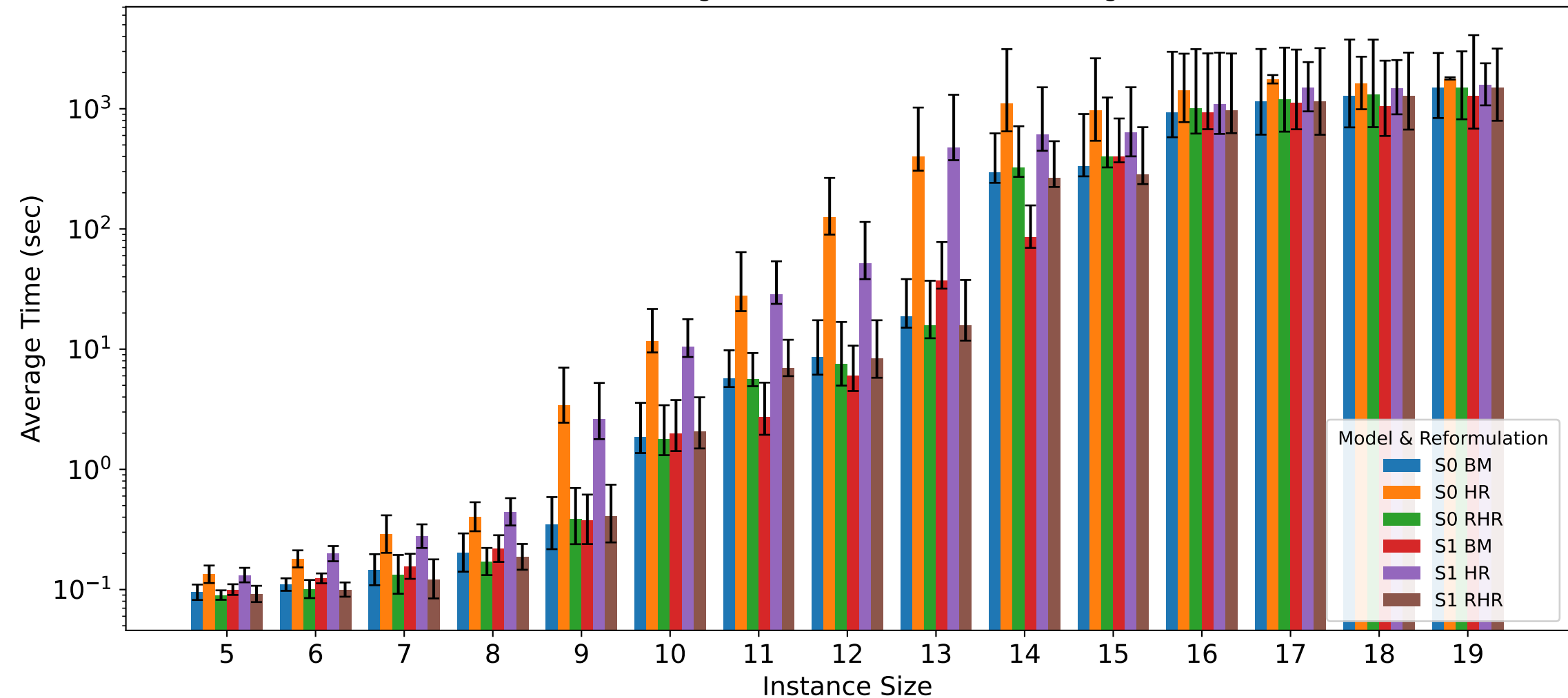
Average Solve Time by Size & Reformulation (10 Cases Averaged; \pm 1 Standard Deviation, Log Scale)
