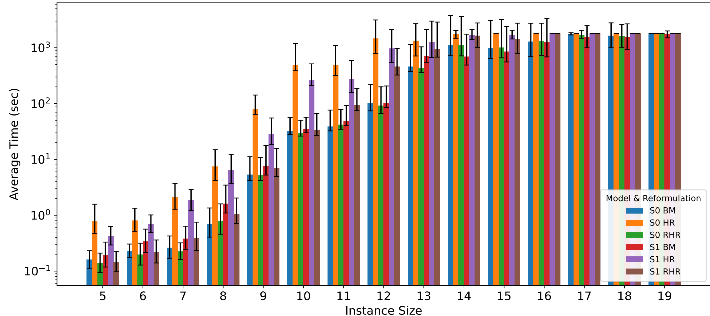
Average Solve Time by Size & Reformulation using SCIP (10 Cases Averaged; \pm 1 Standard Deviation, Log Scale)
