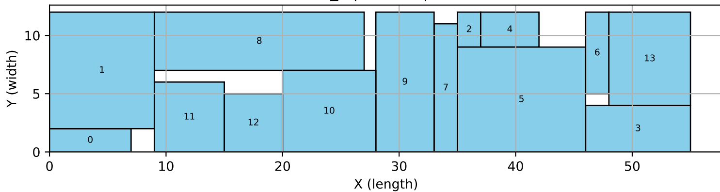
14_3 | altered | hull
