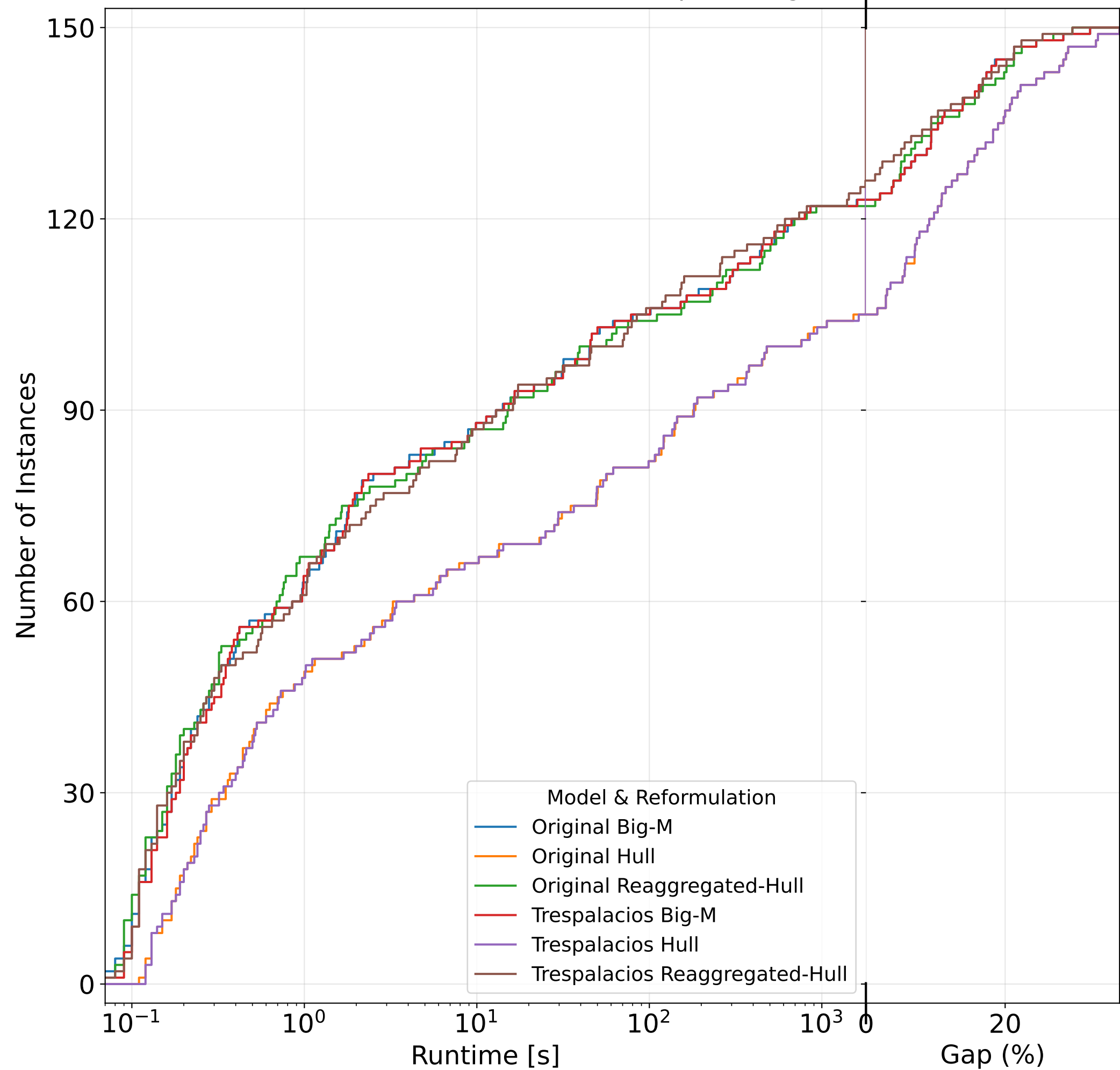
Absolute Performance Profile of Strip Packing Problem
