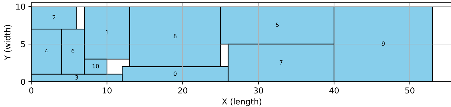
11_2 | tres_sym | hull
