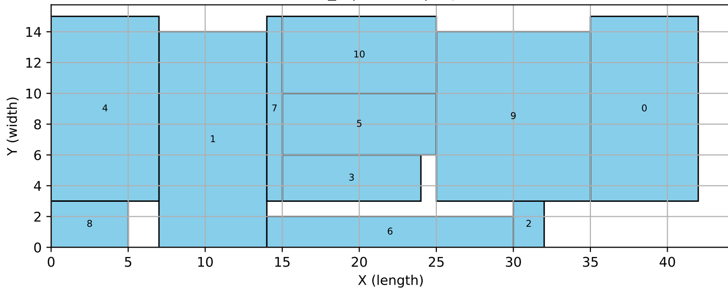
11_5 | altered | bigm
