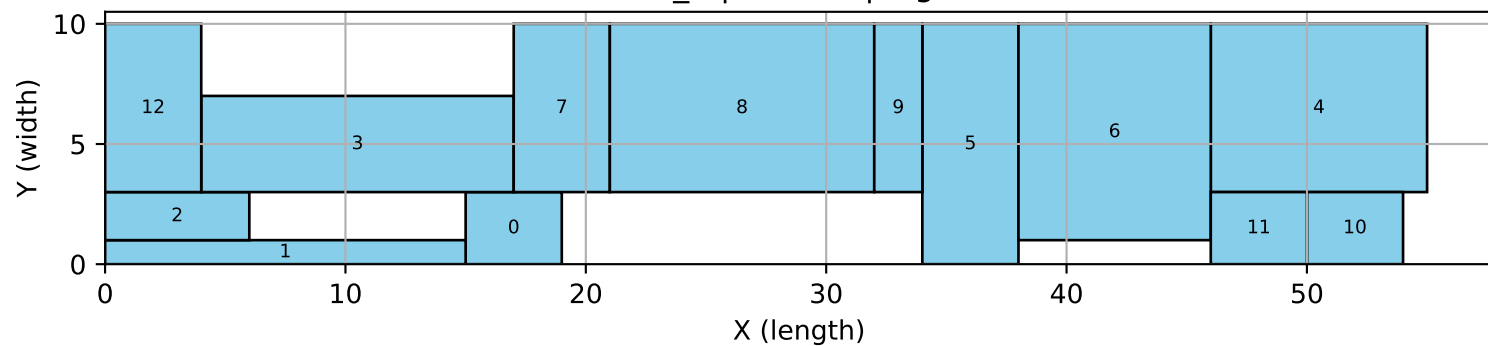
13_2 | altered | bigm
