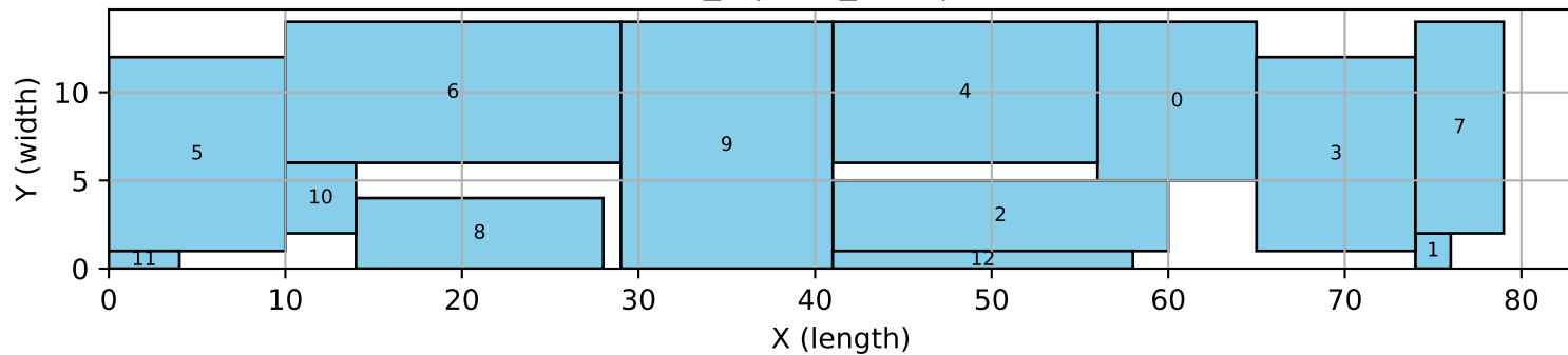
13_7 | tres_sym | hull
