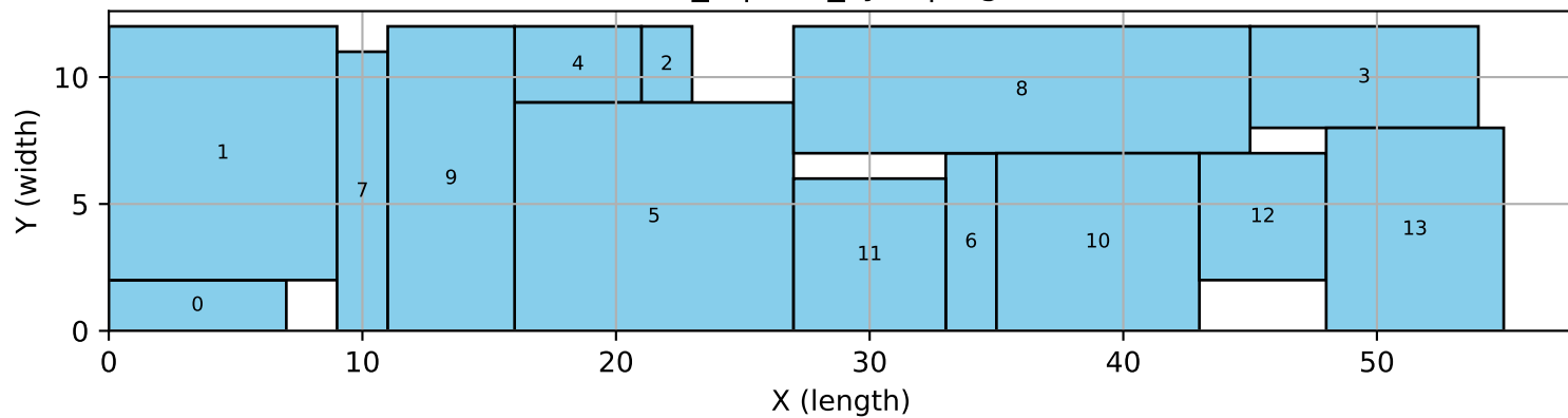
14_3 | tres_sym | bigm
