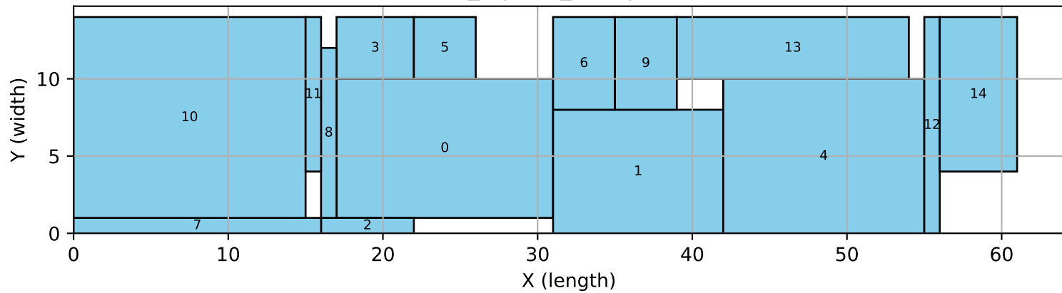
15_4 | tres_sym | bigm
