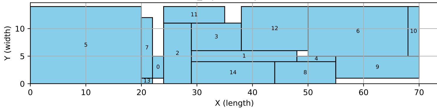
15_8 | altered | bigm
