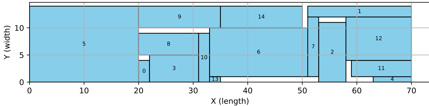
15_8 | traditional | hull
