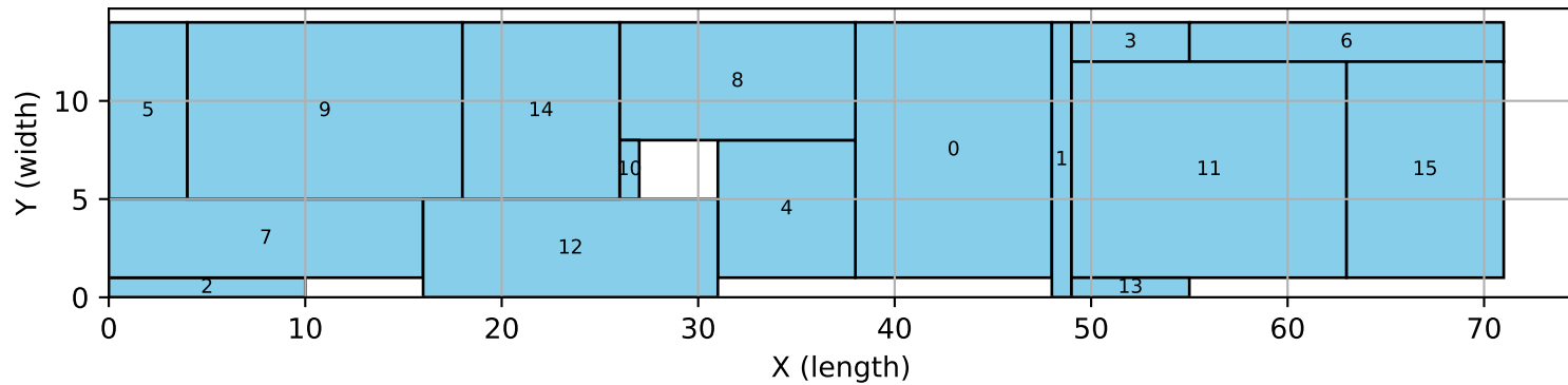
16_4 | traditional | bigm
