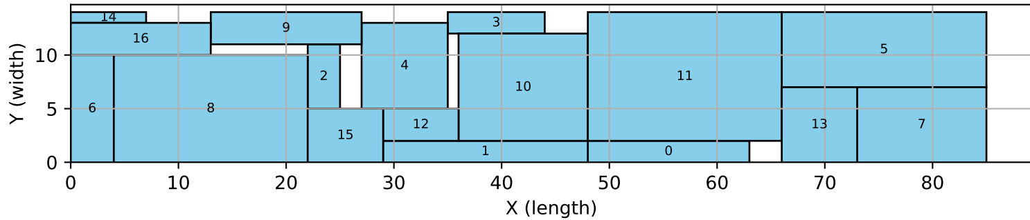
17_7 | traditional | bigm
