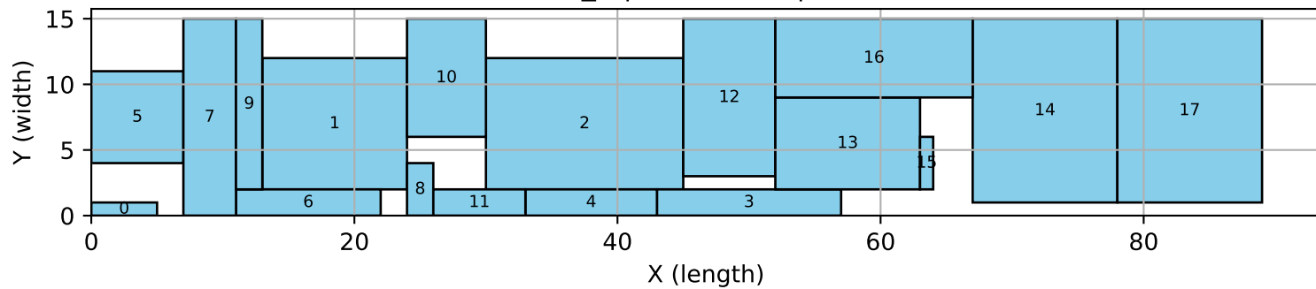
18_5 | traditional | hull
