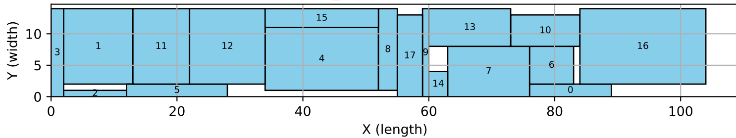
18_6 | altered | bigm
