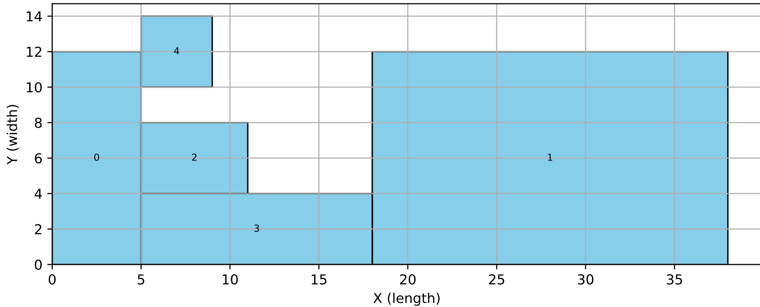
5_9 | reagg | MIP
