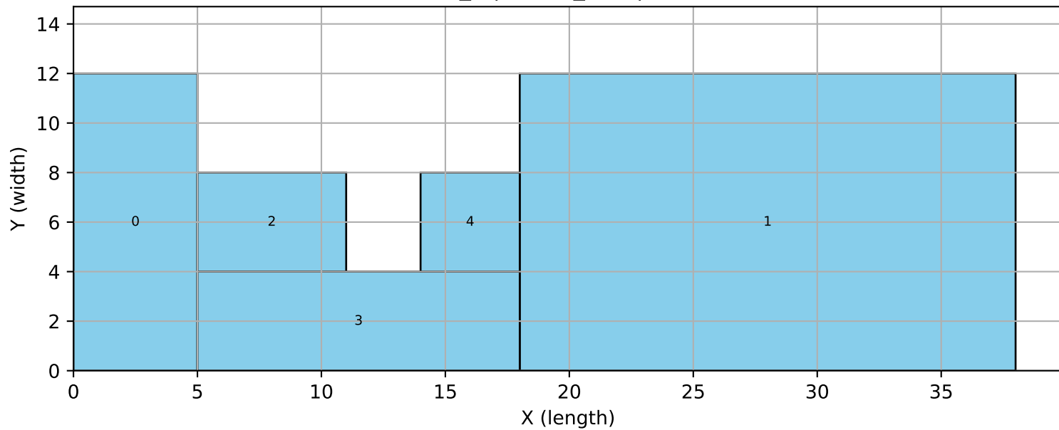
5_9 | reagg_tres | MIP
