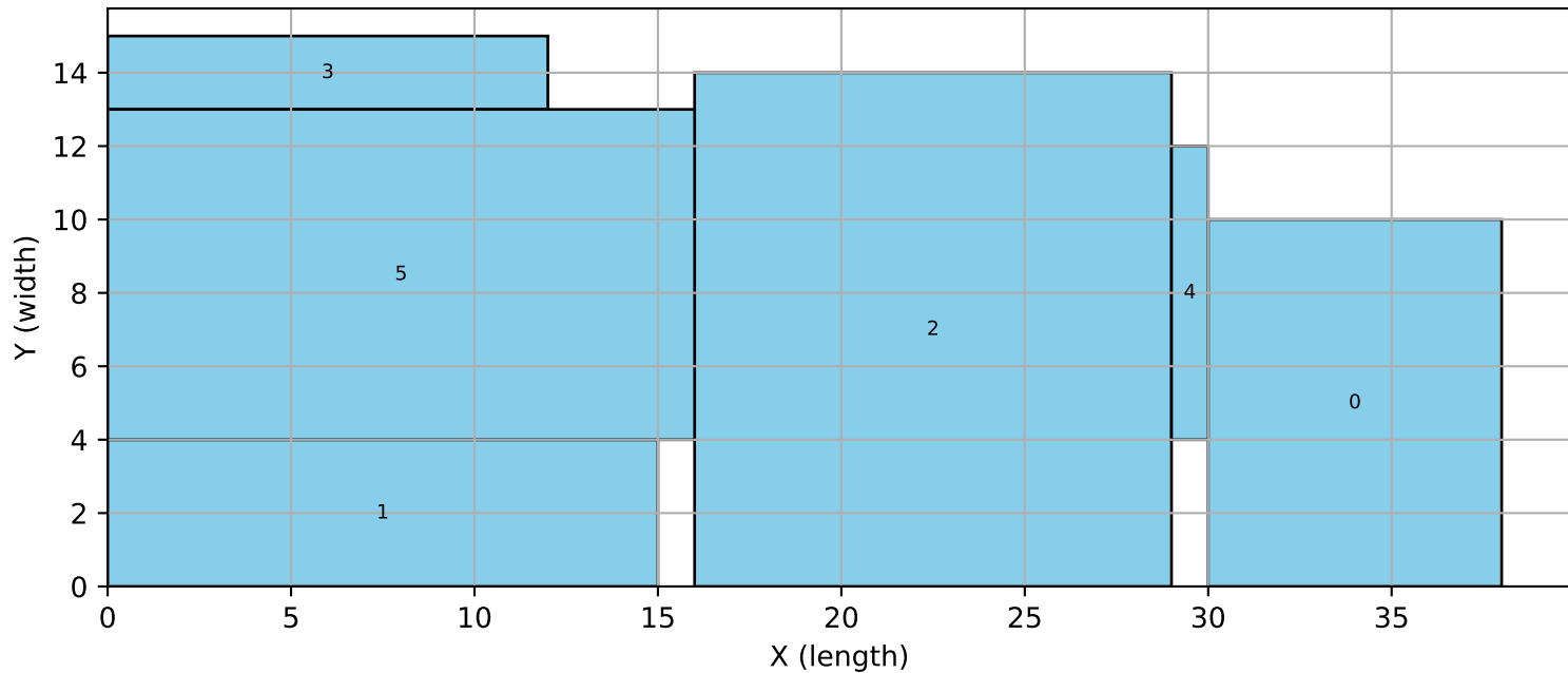
6_4 | reagg | MIP
