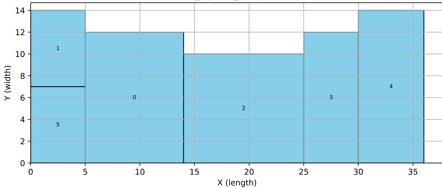
6_5 | tres_sym | hull
