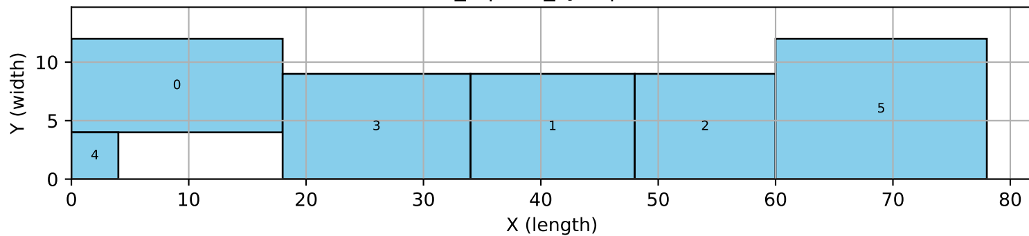
6_6 | tres_sym | hull
